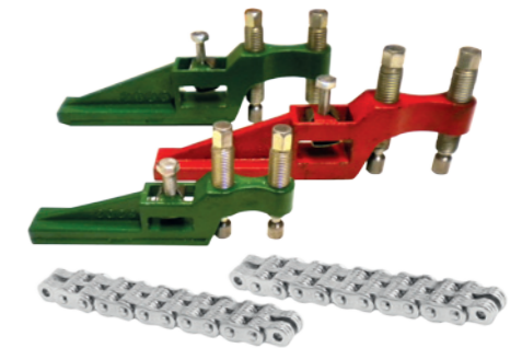
Standard or heavy duty chain is available according to reforming requirements
