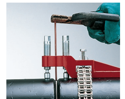
The jackbars are designed to allow clearance around the pipe for any welding torch or rod.
